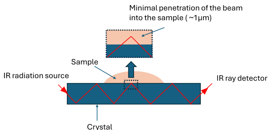
Figure 3.1. The phenomenon of total internal reflection inside the ATR attachment crystal.
