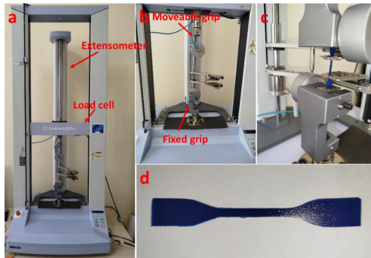
Figure 3.8. Tensile test instrument (a), grips and extensometer (b), mounting of a specimen (c) and specimen for tensile test measurements (d).
