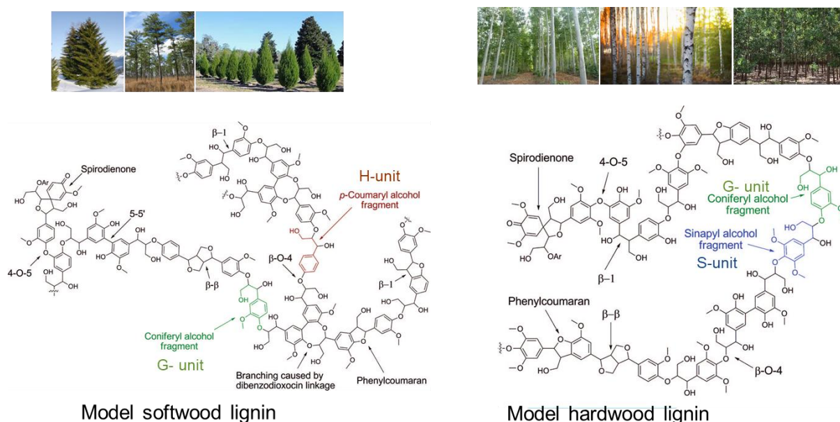
Figure 1.4. Native lignin structure (adopted from Zakzeski et al., 2010; Ralph et al., 2004).
