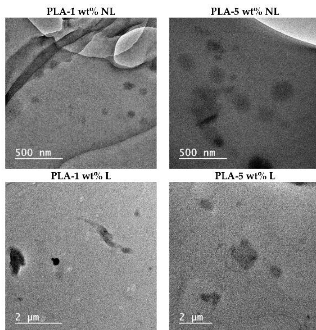
Figure 2.14. TEM micrographs of PLA–L and PLA/NL composites containing 1 and 5 wt% filler (Makri et al., 2022).
