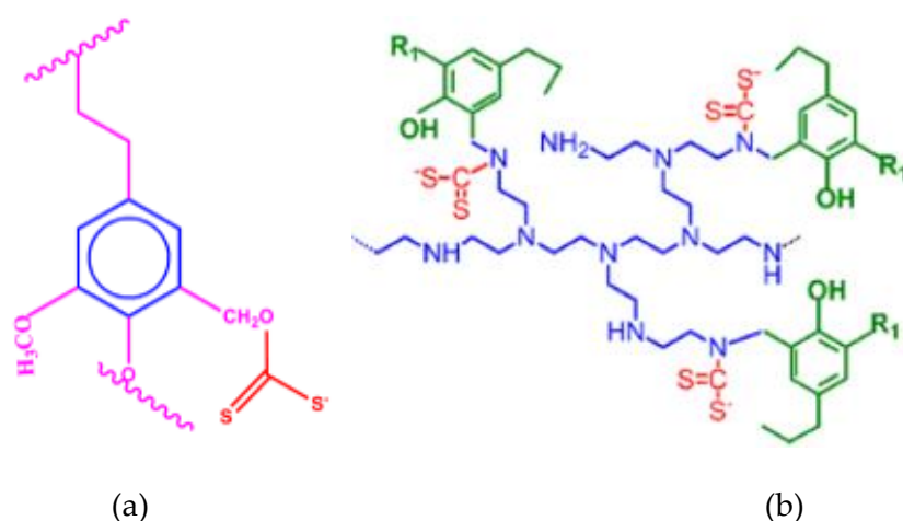
Figure 2.9. Structures of the lignin xanthate resin (a) and surface-functionalized porous lignin with dithiocarbamate groups (b) (from Ge et al., 2014c; Li et al., 2015c).
