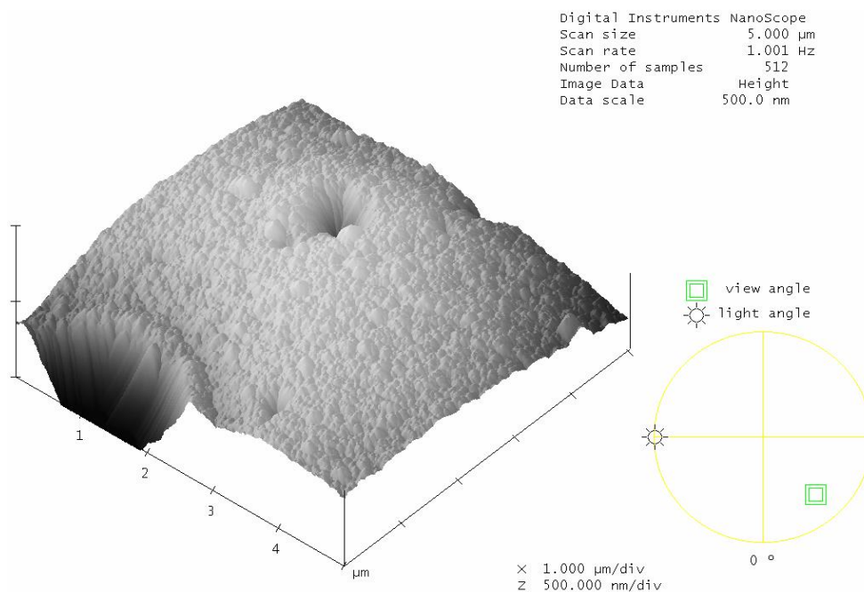
Figure 3.7. Fragment of a DVB copolymer microsphere made with an atomic force microscope (AFM) - magnification x27,000.
