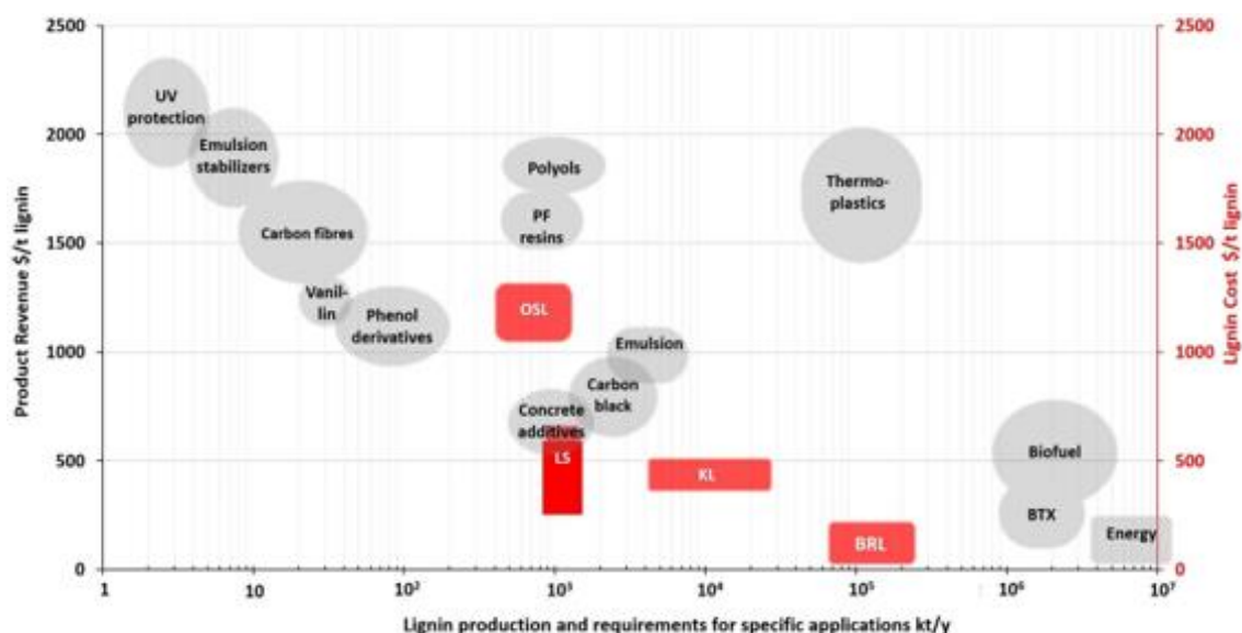
Figure 1.6. Evaluation of lignin market potentials based on publicly available information. Abbreviations: OSL – organosolv lignins, LS – liginosulfonates, KL – Kraft lignins, BRL – (crude) biorefinery lignins (adapted from Balakshin et al., 2021).
