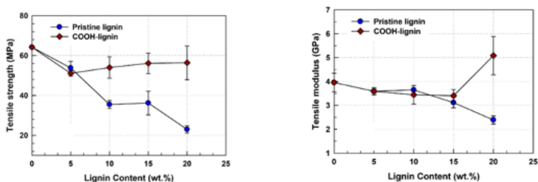
Figure 2.16. Tensile strength and tensile modulus of PLA composites with modified and unmodified lignin (Hong et al., 2021).
