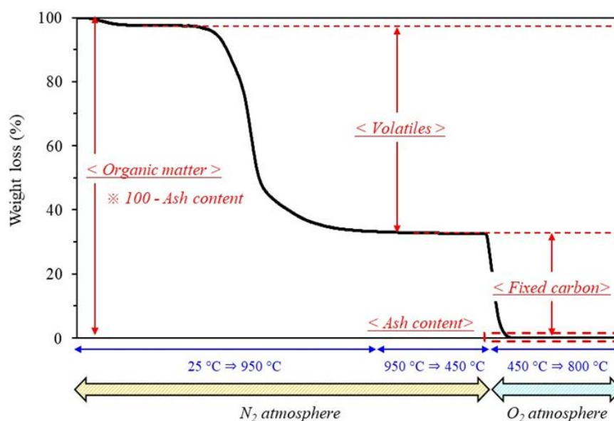
Figure 3.6. Thermogravimetric analysis of lignin (adapted from Tagami, 2018).
