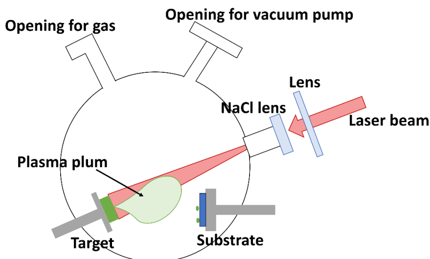
Figure 3.13. Schematic illustration of the reactor for PLA.
