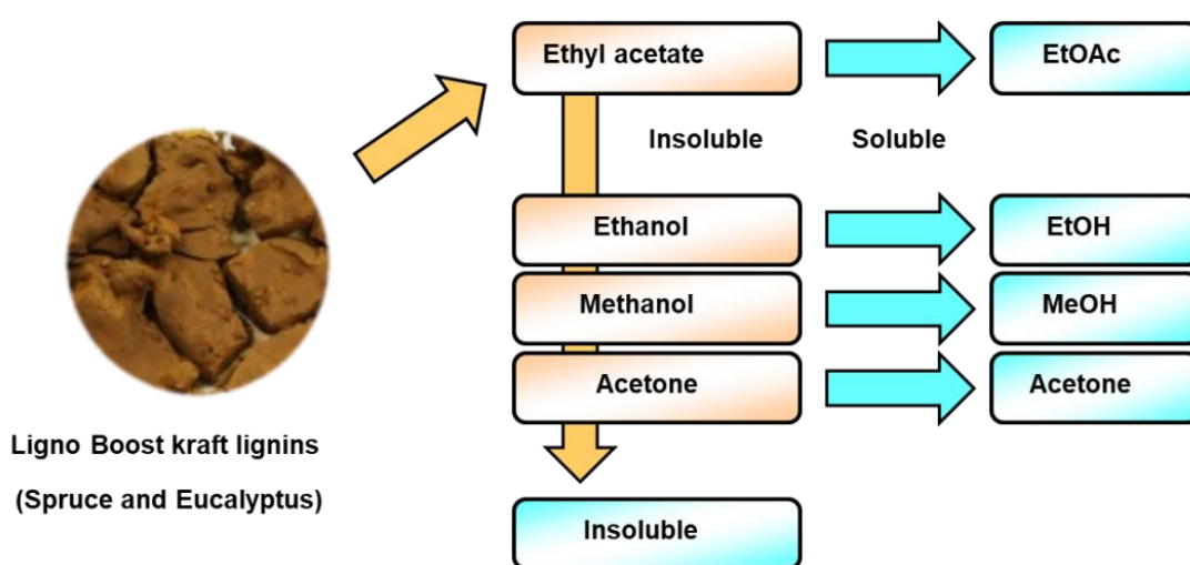
Figure 1.8. Solvent fractionation of lignin: based on differential solubility (adapted from Tagami, 2018).
