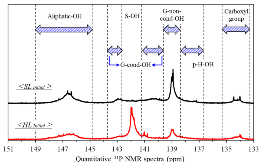
Figure 1.7. Example of ^{31}\text{P} NMR spectra for spruce (SL) and eucalyptus (HL) kraft lignin (adapted from Tagami, 2018).
