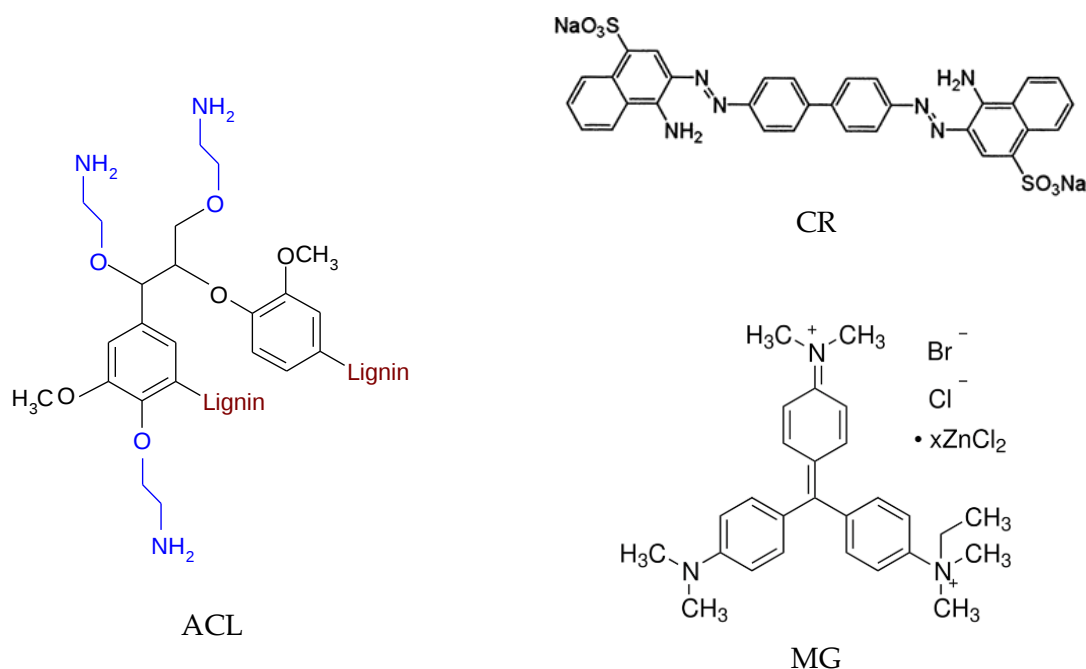
Figure 2.7. Structures of ACL and dyes (CR – Congo Red, MeG – Methylene Green).
