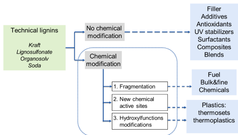
Figure 1.10. Uses of lignin with or without chemical modification (adapted from Laurichesse et al., 2014).
