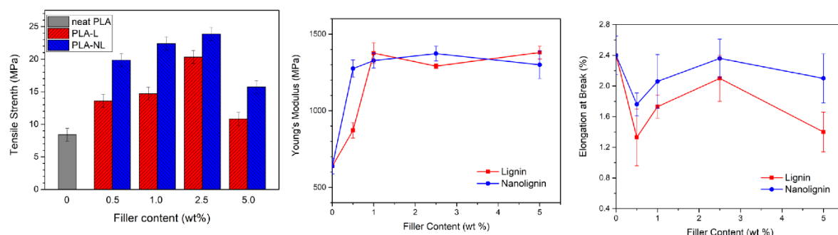
Figure 2.15. Mechanical properties of PLA/L and PLA/NL (Makri et al., 2022).
