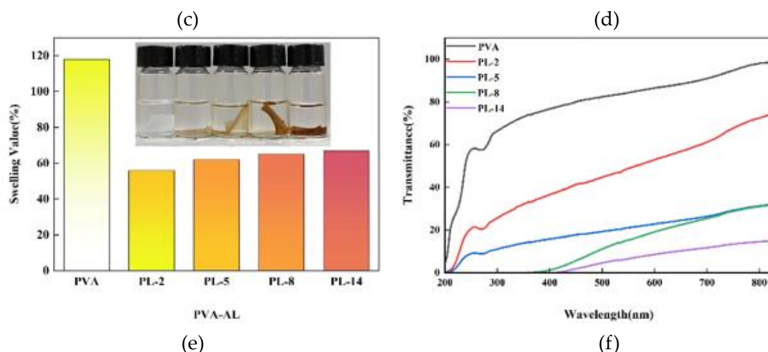
Figure 2.13. Infrared spectra (a), thermogravimetric (b), stress–strain (c), XRD (d), solubility (e), and UV optical resistance (f) of PVA, PL-2, PL-5, PL-8, and PL-14 (Liu et al., 2024).
