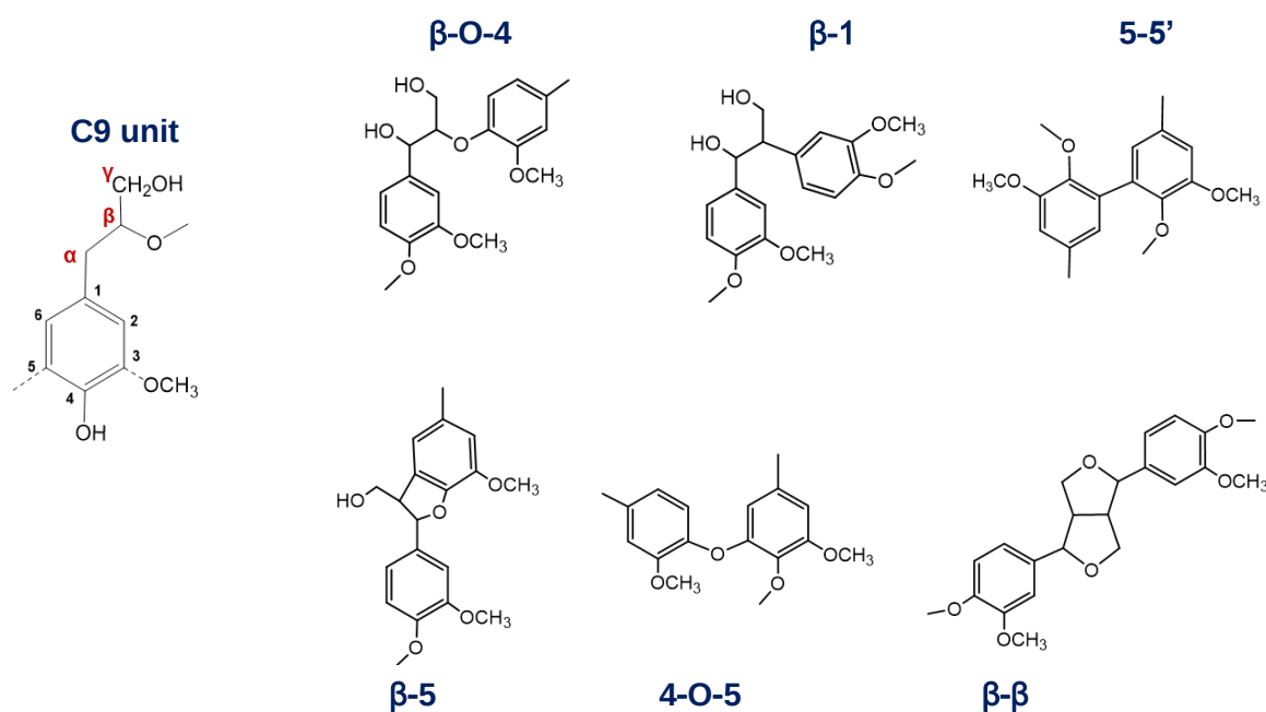
Figure 1.3. Types of interunit linkages in native lignin (Erickson et al., 1973; Nimz, 1974).
