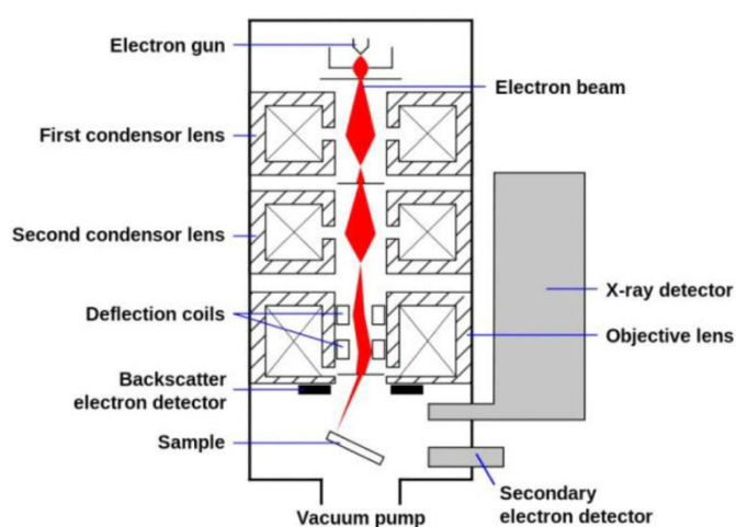
Figure 3.10. Schematic illustration of SEM (Alqaheem and Alomair, 2020).
