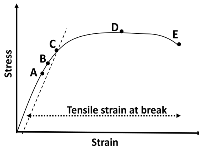
Figure 3.9. Stress-strain curve.
