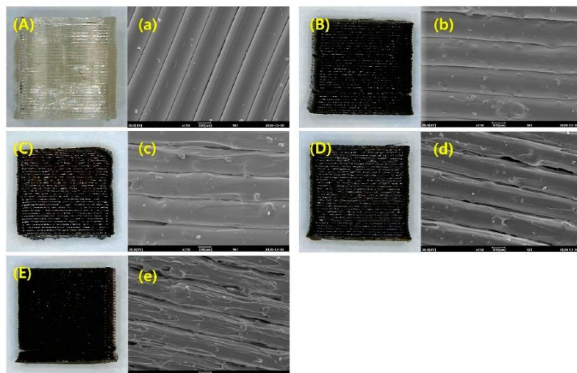
Figure 2.17. Optical image and SEM micrographs of 3D printed objects from PLA (A, a) and PLA-modified lignin with contents of 5 wt.% (B, b), 10 wt.% (C, c), 15 wt.% (D, d), and 20 wt.% (E, e) (Hong et al., 2021).
