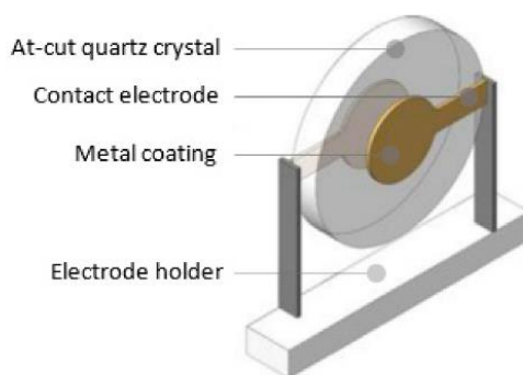
Figure 3.12. Schematic representation of AT-cut quartz crystal, with gold electrodes on both sides of the substrate (Migoń et al., 2020).
