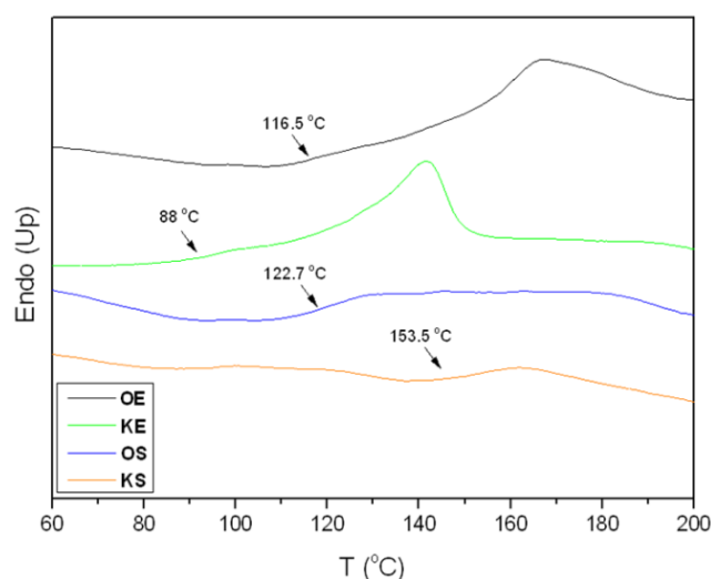
Figure 3.4. T_g 's values for technical lignins: organosolv eucalyptus (OE) and spruce (OS), and kraft eucalyptus (KE) and spruce (KS) (adapted from Gordobil, et al. 2016).
