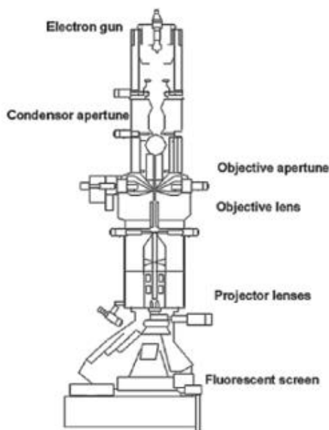
Figure 3.11. Schematic illustration of TEM (Alqaheem and Alomair, 2020).
